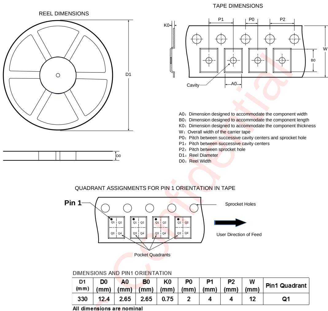
Figure 11 Tape and Reel
