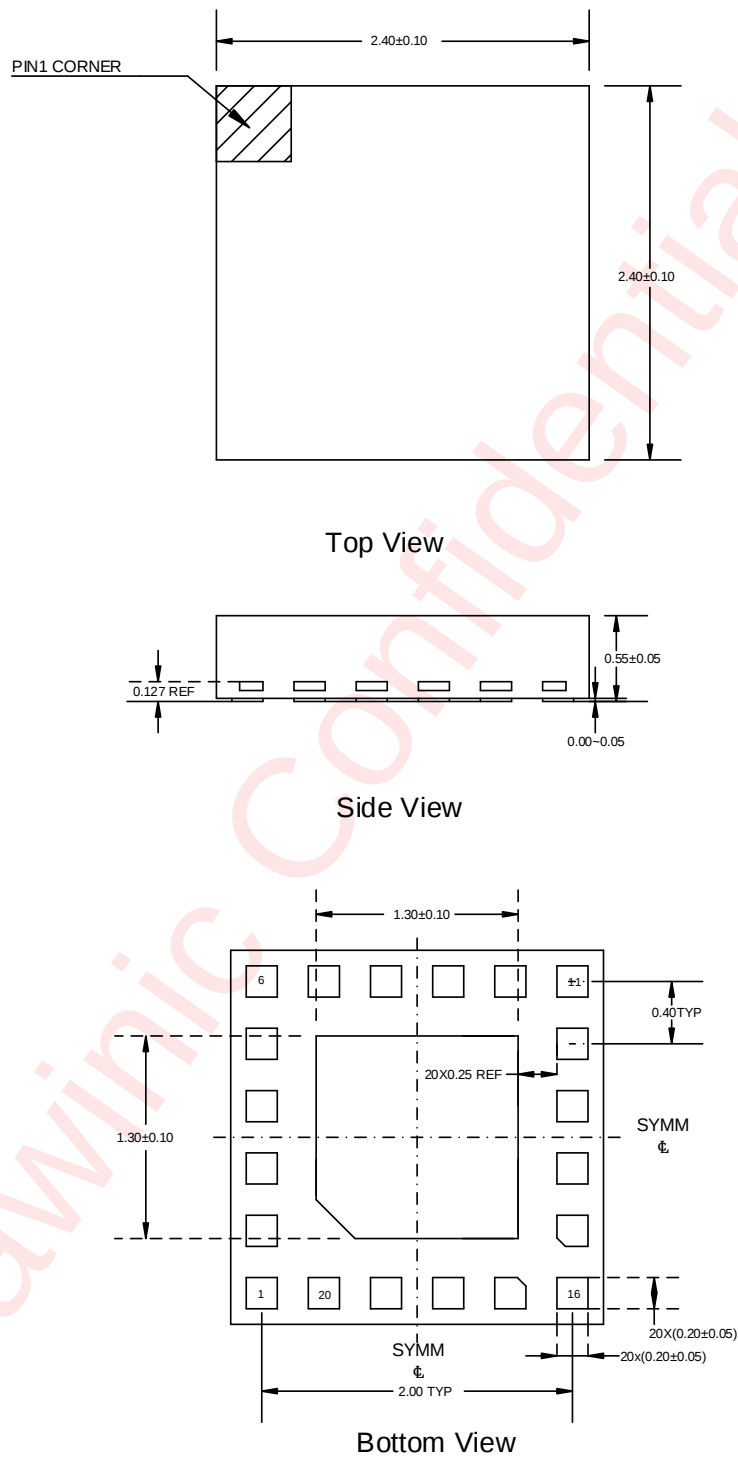
Figure 12 Package Outline
