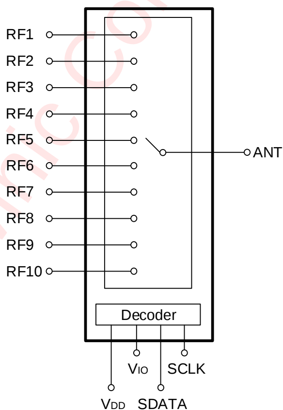
Figure 3 Functional Block Diagram
