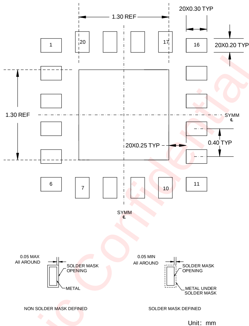
Figure 13 Land Pattern Data
