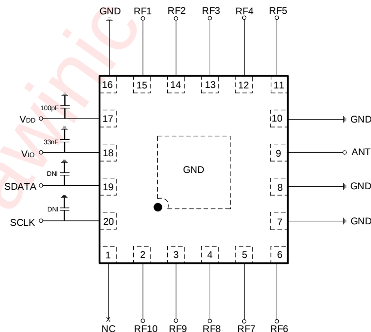
Figure 1 Typical Application Circuit of AW13510
