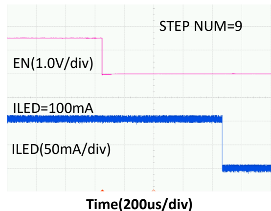
Figure 9. Shutdown Wave
