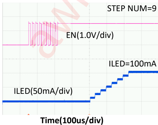
Figure 8. Startup Wave
