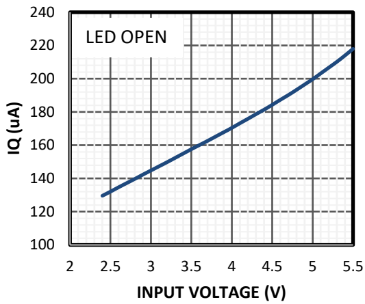
Figure 4. Quiescent Current
