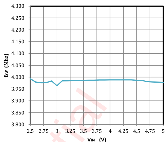
4-MHz Frequency vs Input Voltage
