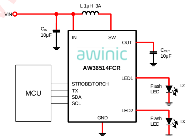
Typical Application Circuit of AW36514
