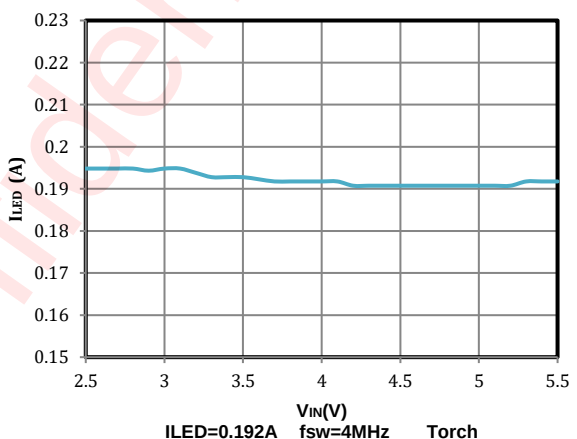
LED1/2 Torch Current vs Input Voltage
