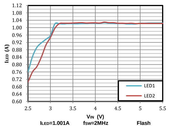
LED1 & LED2 Current vs Input Voltage
