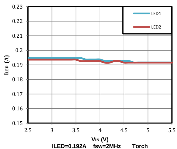
LED1&2 Torch Current vs Input Voltage
