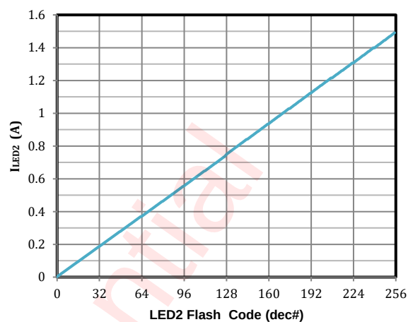
LED2 Flash Current vs Brightness Code
