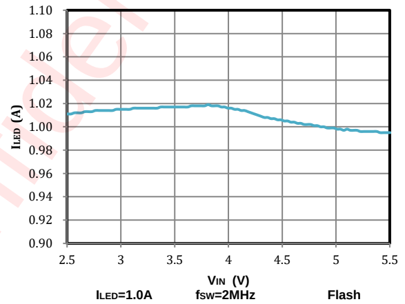
LED1/2 Flash Current vs Input Voltage
