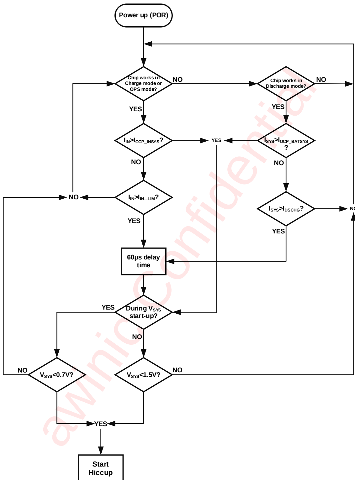
Figure 22 Short Circuit Hiccup Protection Flow Chart
