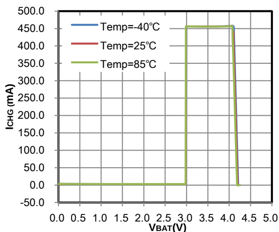
Figure 4 I_{CHG} vs. V_{BAT} , V_{IN}=5.0V
