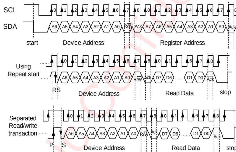
Figure 37 I²C Read Timing
