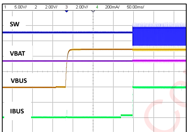
Figure 15 Charge startup at VBUS plug-in
