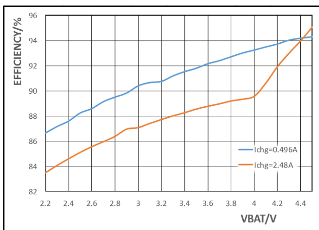
Figure 13 Charge efficiency vs. VBAT
