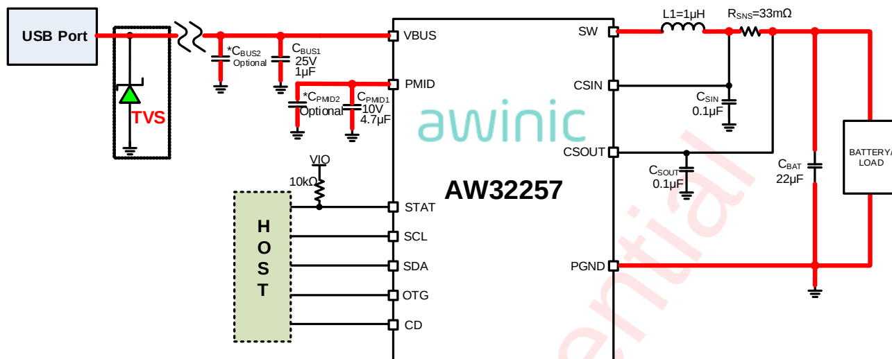
Figure 1 Typical Application Circuit of AW32257
