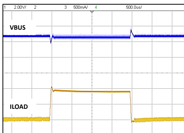
Figure 18 Load transient for boost mode
