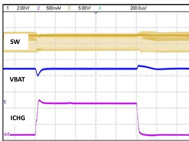
Figure 12 Load transient in download mode
