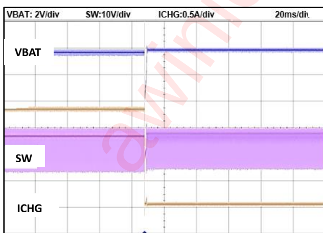
Figure 17 Battery removal during charging
