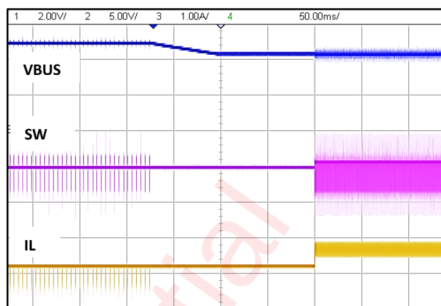
Figure 26 Boost to charge mode transition
