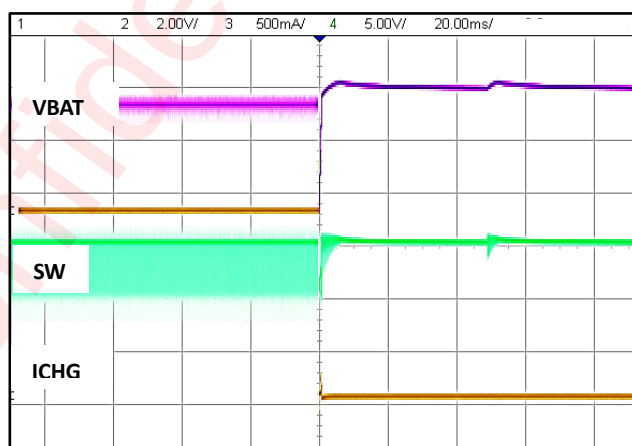
Figure 16 Battery removal during charging
