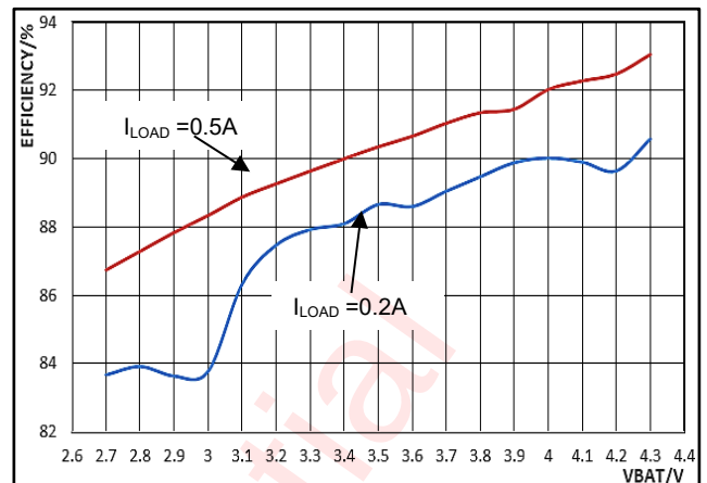
Figure 20 Efficiency for boost mode
