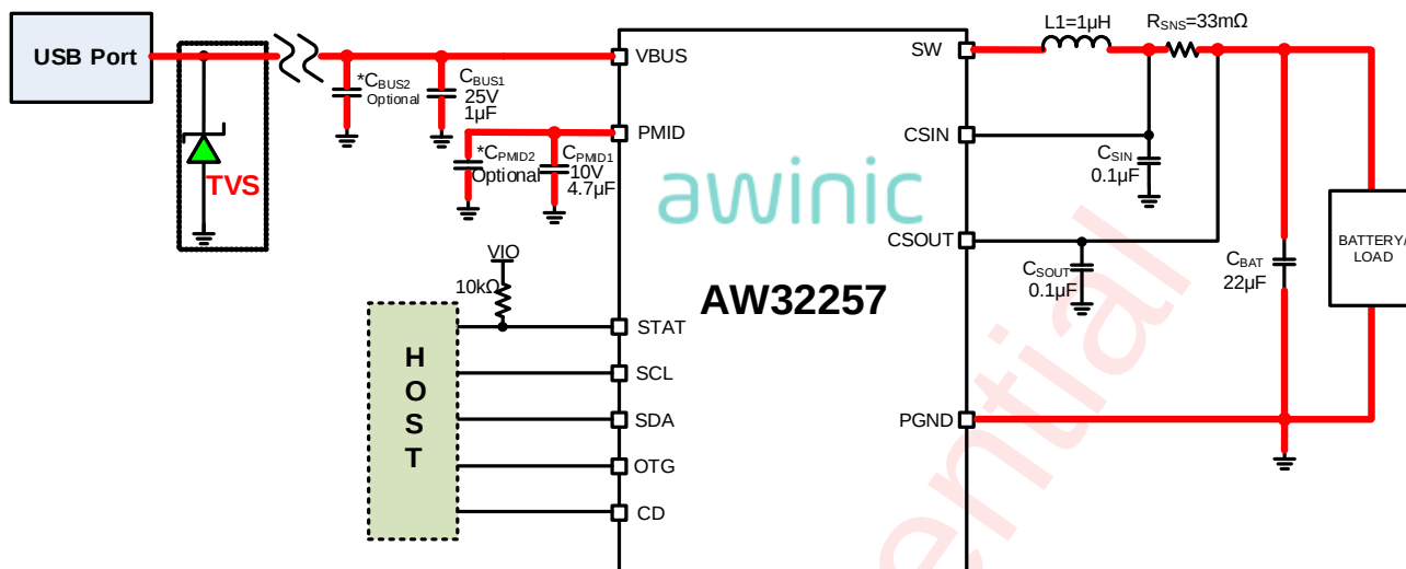
Figure 4 AW32257 Application Circuit
