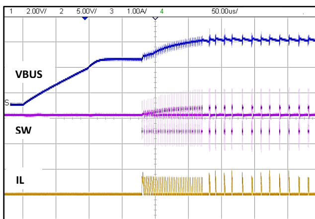
Figure 25 Boost startup
