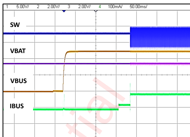
Figure 14 Charge startup at VBUS plug-in
