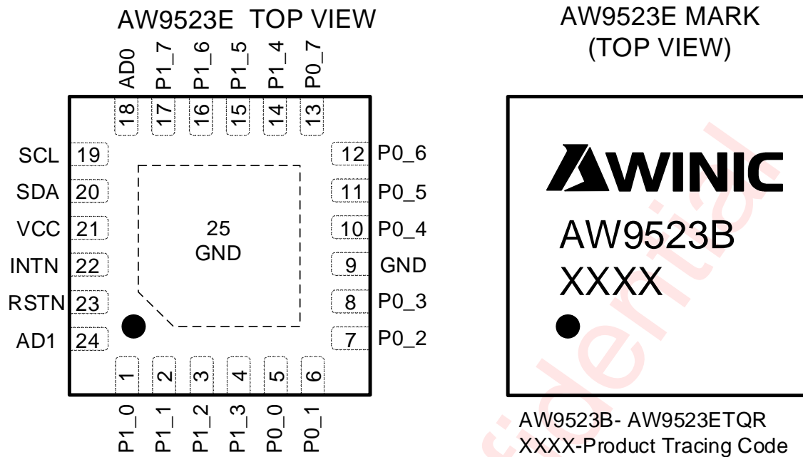
Figure 3 AW9523E PIN CONFIGURATION AND MARKING
