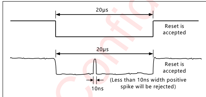
Figure 15 Operation When RSTN SLOW
