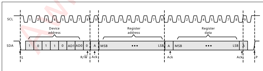
Figure 12 AW9523E Write Operation
