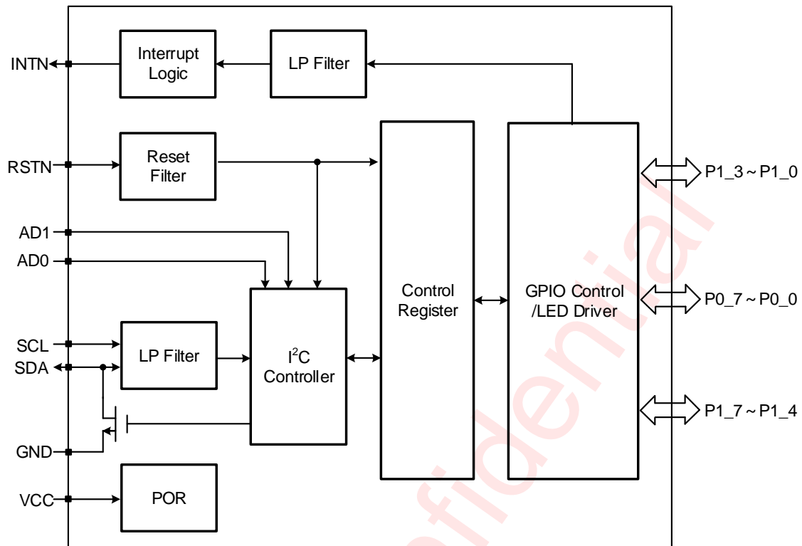
Figure 4 AW9523E Functional Block
