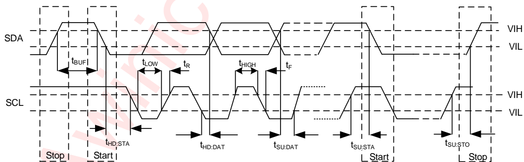
Figure 5 I2C Interface Timing
