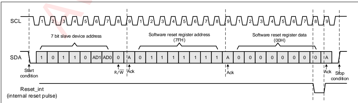
Figure 16 Software Reset Timing
