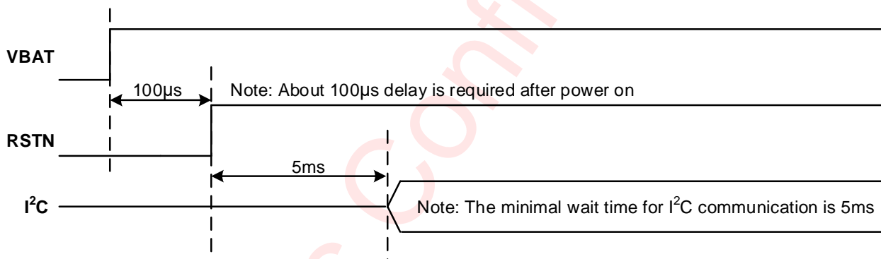
Figure 6 AW9523E Power On
