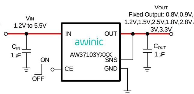
Fixed Output Voltage Application with SNS
