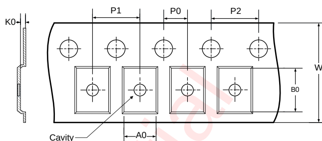
TAPE DIMENSIONS
