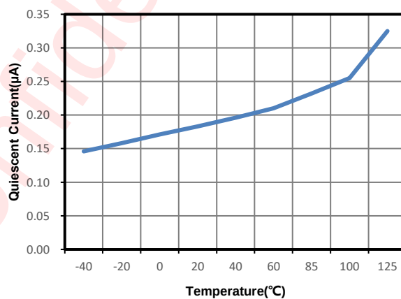
IQ_VIN vs TEMP
