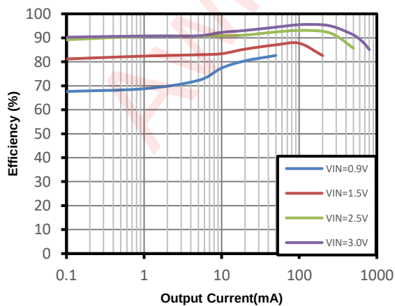
AW360994 Load Efficiency with Different Inputs
