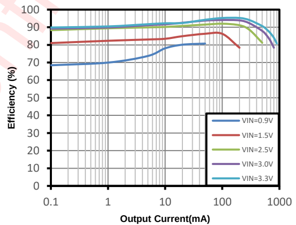
AW360995 Load Efficiency with Different Inputs
