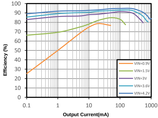
AW36099 V_{OUT} = 5\text{V} Load Efficiency with Different Inputs
