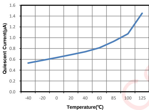
IQ_VOUT vs TEMP
