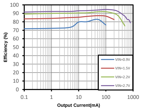
AW360993 Load Efficiency with Different Inputs
