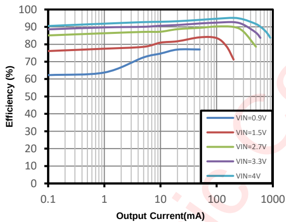
AW360996 Load Efficiency with Different Inputs
