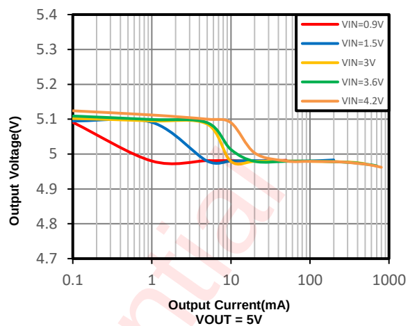
Load Regulation
