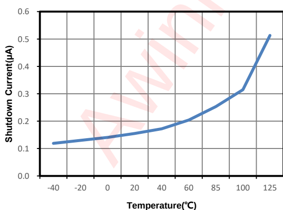
ISD vs TEMP
