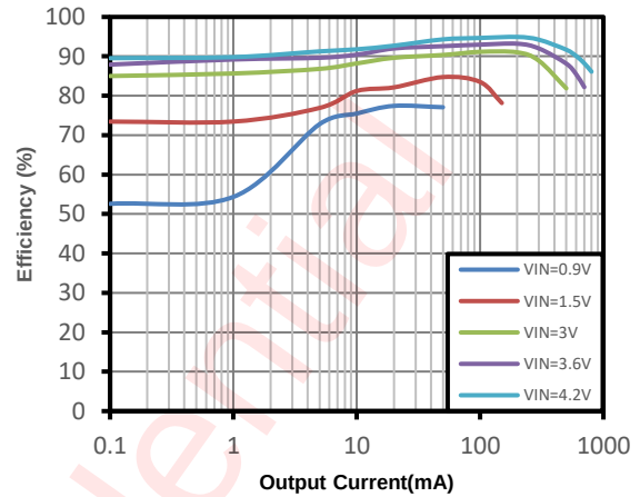
AW360997 Load Efficiency with Different Inputs
